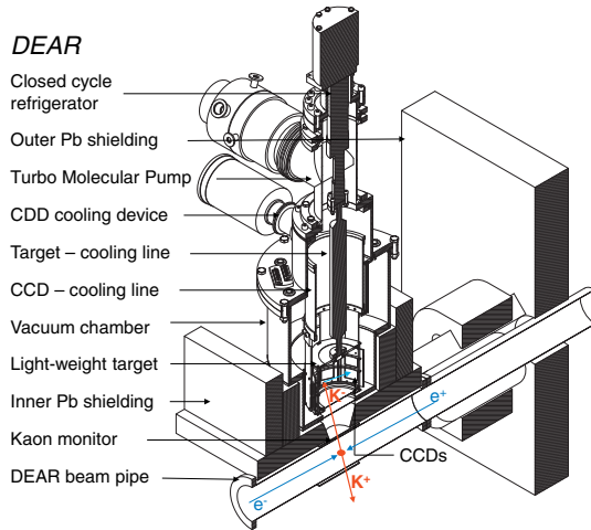
FIG. 16. Schematic view of the DEAR experimental setup; only the right outer lead wall shielding is shown.
