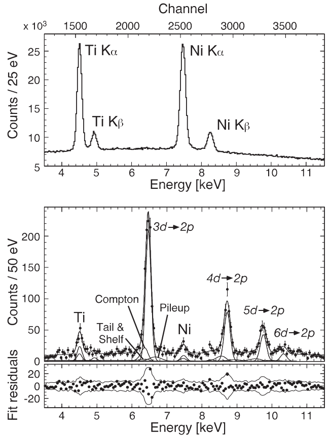
FIG. 23. The SDD kaonic helium-4 spectra (top) without and (bottom) with stopped K^- -triggered events. From Okada et al. , 2007.
