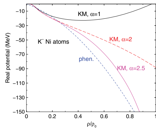
FIG. 41. Real part of the best fit K^- -Ni optical potential based on the single-nucleon amplitudes plus a phenomenological multi-nucleon amplitude B(\rho/\rho_0)^\alpha . Shown for comparison as short-dashed lines is a purely phenomenological potential (Friedman and Gal, 2007). Adapted from Friedman et al. , 2017.
