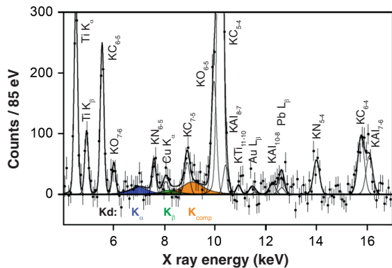
FIG. 33. X-ray spectrum of the exploratory kaonic deuterium measurement. The continuous background fit component is already subtracted. The fit was performed with fixed Kd transition shift and width ( -805, 750 eV) and fixed yield ratios of the K transitions. The integrated luminosity was 100 \text{ pb}^{-1} . The lines from kaonic x rays generated by kaons stopping in the window foils as well as the fluorescence lines excited by background are labeled. Note the excess of events in the region of a possible signal. From Bazzi et al. , 2013.
