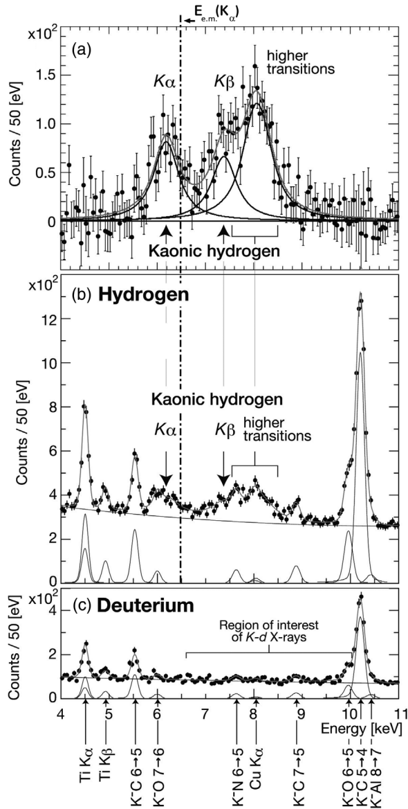
FIG. 27. The global simultaneous fit of the x-ray energy spectra of hydrogen and deuterium data. (a) Residuals of the measured kaonic-hydrogen x-ray spectrum after subtraction of the fitted background, clearly displaying the kaonic-hydrogen K -series transitions. The fit components of the K^-p transitions are also shown, where the sum of the functions is drawn for the higher transitions (greater than K_\beta ). (b), (c) Measured energy spectra with the fit lines. Fit components of the background x-ray lines and a continuous background are also shown. The dot-dashed vertical line indicates the e.m. value of the kaonic-hydrogen K_\alpha energy. From Bazzi et al., 2011a .
