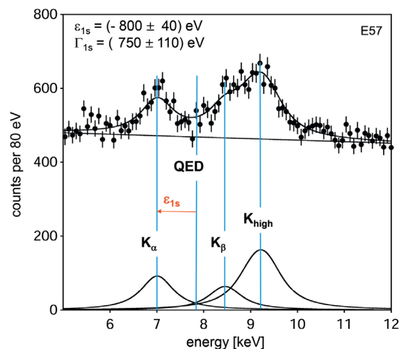
FIG. 38. Simulated E57 kaonic deuterium spectrum, assuming a shift \varepsilon_{1s} = -800 \pm 40 eV and width \Gamma_{1s} = 750 eV of the 1s state, as well as a K_\alpha yield of 10^{-3} .
