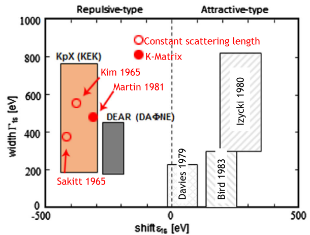
FIG. 15. The shift and width obtained by the KpX experiment are compared with the results of three previous measurements (Davies et al. , 1979; Izycki et al. , 1980; Bird et al. , 1983) and with some of the analyses of the low-energy \bar{K}N scattering data (Kim, 1965; Sakitt et al. , 1965; Martin, 1981). The DEAR result (Beer et al. , 2005) is also reported.
