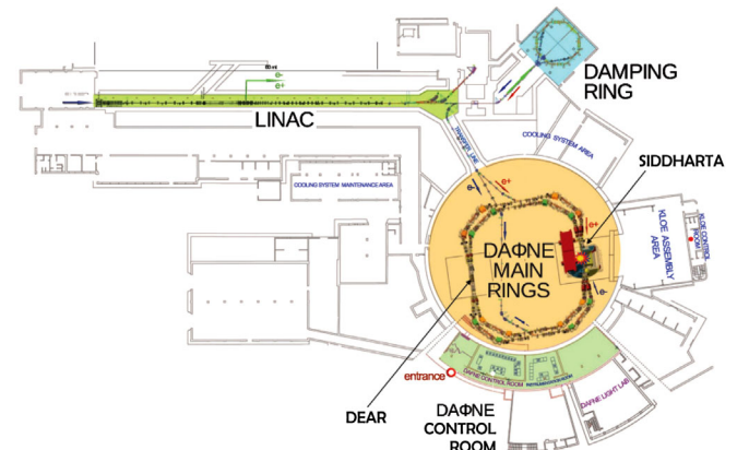
FIG. 3. DAΦNE accelerator complex layout. Adapted from Vignola et al. , 1996.
