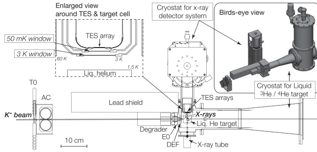
FIG. 39. A cross-section top view of the J-PARC E62 experimental setup. The inset shows a birds-eye view around TES and the helium target cell. A set of beam detectors, a cryogenic liquid helium-3 and helium-4 target system, and the NIST's TES x-ray spectrometer system are shown. From Okada, 2015.
