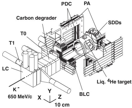
FIG. 22. Closeup of the E570 experimental setup (see the Fig. 21 caption).
