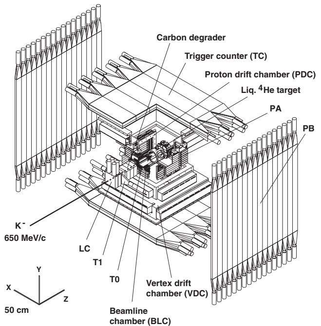
FIG. 21. Schematic drawing of the E570 experimental setup. The z axis is the beam direction, the x axis is the horizontal axis (the left of the beam view is positive), and the y axis is the vertical one (the top is positive). The 650-MeV/c negatively charged kaon beam is degraded by carbon layers and stopped in a superfluid liquid helium-4 target. Characteristic x rays generated from a kaonic-helium atom are measured by SDDs installed downstream of the target. LC: Lucite Cerenkov counter. T1 and T0: scintillation counters. BLC: beam line drift chamber. VDC: vertex drift chamber. PDC: proton drift chamber. TC: scintillation counter for the VDC. PA and PB: scintillation counters for the PDC.
