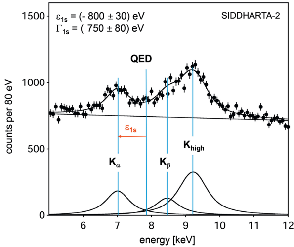
FIG. 36. Simulated SIDDHARTA-2 kaonic deuterium spectrum, assuming a shift \varepsilon_{1s} = -800 \pm 30 eV and width \Gamma_{1s} = 750 eV of the 1s state, as well as a K_\alpha yield of 10^{-3} . The spectrum was simulated for an integrated luminosity of 800 \text{ pb}^{-1} .
