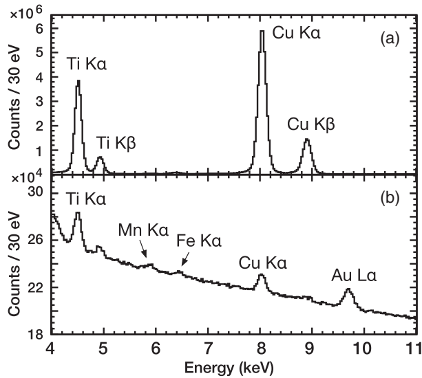
FIG. 29. X-ray energy spectra of the SDDs, where data of all the selected SDDs were summed: (a) data taken with the x-ray tube in the calibration runs, and (b) data uncorrelated to the kaon triggers in the production runs. The peak positions of the titanium, copper, and gold fluorescence x-ray lines in (b) were used to determine the uncertainty on the energy calibration and the energy dependence of the energy resolution. From Bazzi et al. , 2011c .
