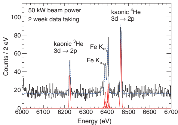
FIG. 40. Expected spectrum in the J-PARC E62 experiment. The red lines represent various x-ray components, and the blue dotted line represents a fit to the spectrum assuming as an example a constant background. From Okada, 2015.
