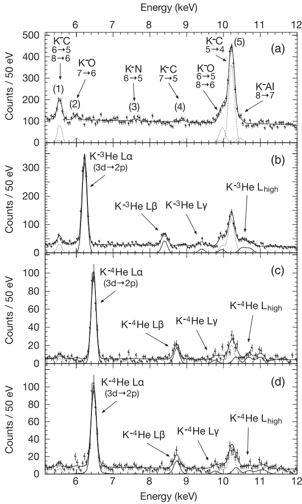
FIG. 31. X-ray energy spectra of different SIDDHARTA target data in the synchronous time window. (a) Deuterium (2.50 g/l), (b) helium-3 (0.96 g/l), (c) helium-4 (1.65 g/l), and (d) helium-4 (2.15 g/l). Several kaonic atom x-ray peaks are indicated by numbers for the deuterium target data: (1) kaonic carbon ( K^-C ) 8 \rightarrow 6 and 6 \rightarrow 5 , (2) kaonic oxygen ( K^-O ) 7 \rightarrow 6 , (3) kaonic nitrogen ( K^-N ) 6 \rightarrow 5 , (4) ( K^-N ) 7 \rightarrow 5 , (5) ( K^-O ) 8 \rightarrow 6 and 6 \rightarrow 5 , ( K^-C ) 5 \rightarrow 4 , and kaonic aluminum ( K^-Al ) 8 \rightarrow 7 transitions. The fit lines in the energy spectra are also shown. The dotted lines show the fit functions of the other kaonic atom x-ray lines produced in the Kapton foils and the aluminum frames. The solid lines show the fit functions of the kaonic-helium x-ray lines in (b), (c), and (d). The background was fitted with a second order polynomial function. The positions of the kaonic-helium x-ray lines in (b), (c), and (d) are indicated by arrows. Adapted from Bazzi et al. , 2014 .
