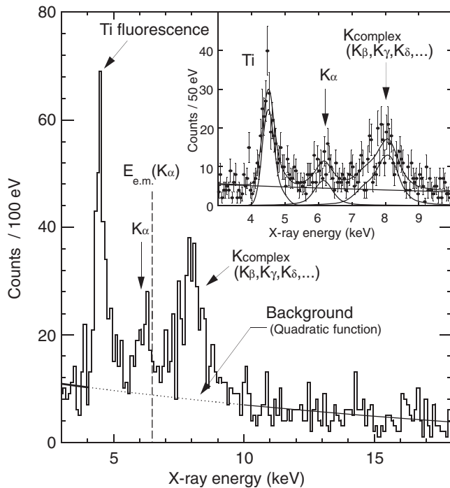
FIG. 14. The x-ray spectrum obtained by the KpX experiment. The inset is a close-up spectrum of the region of interest, together with the fit result. From Iwasaki et al. , 1997.
