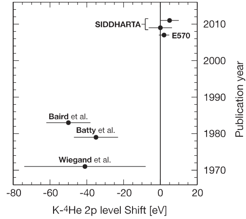
FIG. 32. Comparison of experimental results for the strong-interaction shift of the kaonic helium-4 2p level. The plots exhibit results for the three old experiments ( Wiegand and Pehl, 1971 ; Batty et al. , 1979 ; Baird et al. , 1983 ) and the recent two experiments E570 ( Okada et al. , 2007 ) and SIDDHARTA publishing two values using different datasets in 2009 ( Bazzi et al. , 2009 ) and in 2011 ( Bazzi et al. , 2011c ). The error bars correspond to quadratically added statistical and systematic errors.
