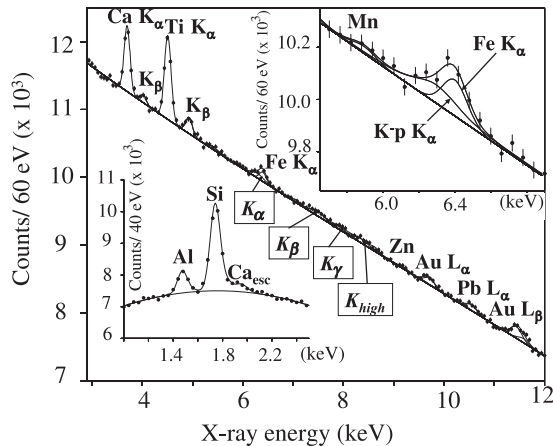
FIG. 17. The measured kaonic-hydrogen x-ray spectrum in the DEAR experiment. The kaonic-hydrogen transitions (indicated by boxes) and the electronic excitations coming from setup materials are visible. The fit functions (total and components) are shown. Upper-right inset: zoom of the kaonic-hydrogen K_\alpha transition region with the continuous background; the iron K_\alpha and the kaonic-hydrogen K_\alpha lines are disentangled. Lower-left inset: zoom of the silicon peak region with the aluminum, silicon, and calcium escape peaks. From Beer et al. , 2005.
