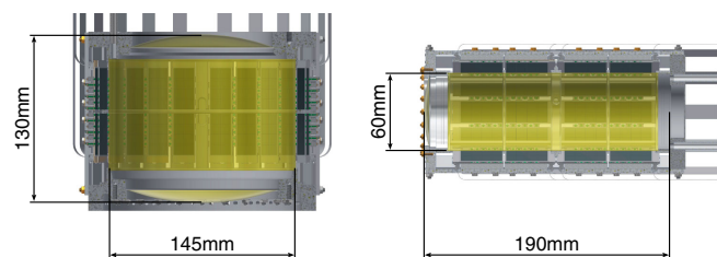
FIG. 34. Sketch of the (left) SIDDHARTA-2 and the (right) E57 cryogenic target cells.
