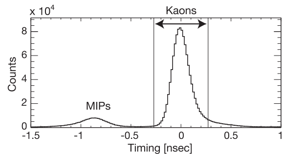
FIG. 26. Kaon identification using the timing of the coincidence signals in the kaon detector with respect to the rf signal of 368.7 MHz from DAΦNE. From Bazzi et al. , 2011a.
