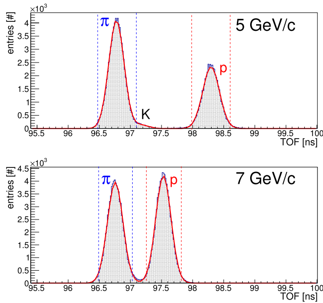
Figure 93. Time difference between the two TOF stations, separated by 29 m flight distance, for beam momenta of 5 GeV/c (top) and 7 GeV/c (bottom). The dashed lines indicate the two selection windows.
