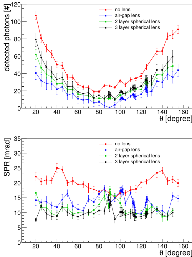
Figure 100. Photon yield (top) and SPR (bottom) as a function of the track polar angle for the narrow bar and various focusing options for tagged protons with a momentum of 7 \text{ GeV}/c . The error bars correspond to the RMS of the distribution in each bin.
