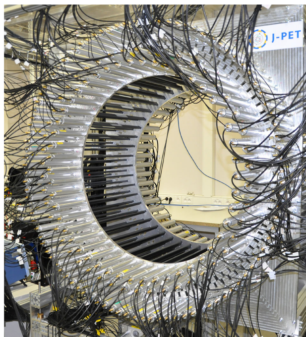
Fig. 1 Photo of the J-PET detector. The inner part of the detector is of a cylindrical shape with the length of 50 cm and diameter of 85 cm. The detector is made of three layers of plastic scintillator strips (black) and readout by vacuum tube photomultipliers (gray)
