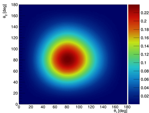
Fig. 10 Visibility \mathcal{V}^2 as a function of the scattering angles \theta_1 and \theta_2
