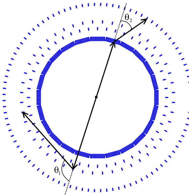
Fig. 2 Cross section of the updated J-PET detector. Superimposed arrows indicate primary and scattered momenta of photons originating from para-positronium decaying in the center of the detector. Detector is build from plastic scintillators strips arranged axially in four rings with radii of 362 mm, 425 mm, 467.5 mm, 575 mm
