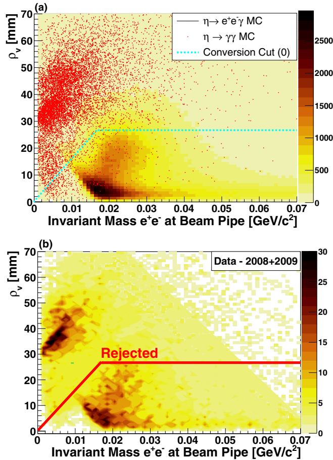
FIG. 7. Condition on conversion suppression shown for (a) simulations and (b) data. For the simulations, the multicolored plot is for the \eta \rightarrow e^+e^-\gamma signal while the red dots are for \eta \rightarrow \gamma\gamma where a photon converts in the beam pipe. The demarcation lines shown in each plot are the same.
