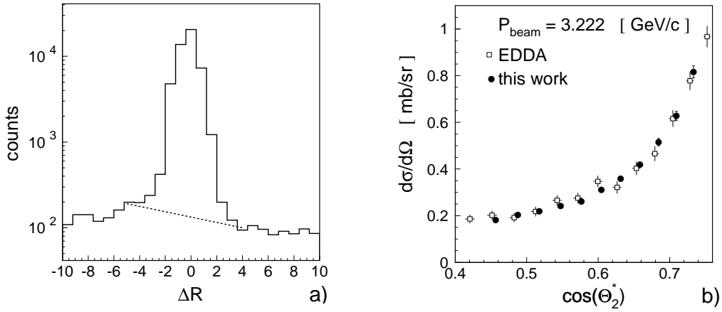
Figure 7.3: (a) Projection of the data from Figure 7.2b along the expected correlation line. The dashed line indicates the estimation of a background. (b) Differential cross section for the elastic proton-proton scattering measured at the beam momentum of P_{\text{beam}} = 3222 \text{ MeV}/c . Cross sections measured by the EDDA collaboration are shown by open squares [125]. Full circles indicate the result of the present work. The points from this work are fitted in the overall normalization to the cross section measured by EDDA. To be better distinguishable both the EDDA data and the points from this work were shifted in the horizontal direction from each other by a half size of the point.
