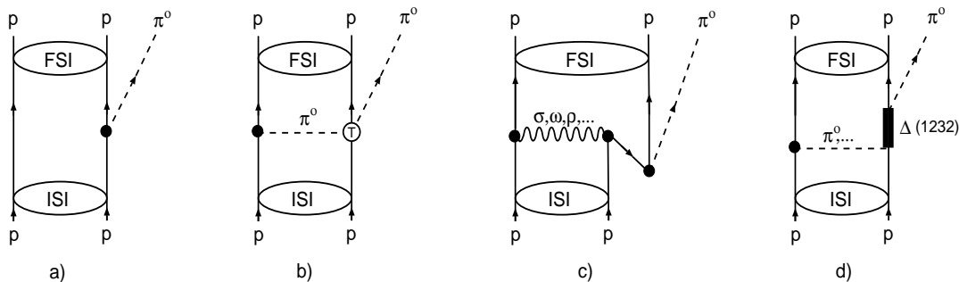
Figure 3.1: Feynman diagrams for the pp \rightarrow pp\pi^0 reaction near threshold: (a) direct term, (b) rescattering term, (c) production through the heavy-meson exchange, (d) resonant term, “ISI” and “FSI” denote proton-proton initial and final state interaction, respectively.
