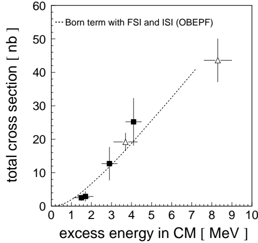
Figure 11.3: Total cross section for the pp \rightarrow pp\eta' reactions as a function of excess energy Q . The dashed curve presents the result of the calculation where only the direct production was considered. Experimental points are taken from: this work (filled squares), and SPES3 [20](open triangles).
