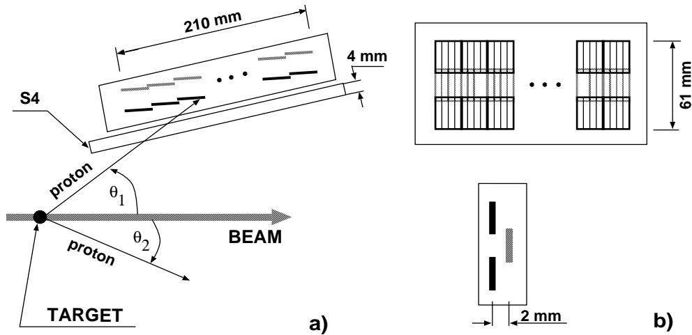
Figure 5.9: (a) Top view of the silicon pad detector (compare Figure 4.1). Each element contains four separate pads with dimensions 22. \times 4.5 \times 0.28 \text{ mm}^3 . The overlap between the detection elements allows to avoid insensitive areas. (b) Silicon pad detector as seen from the target point (above). Side view (below).
