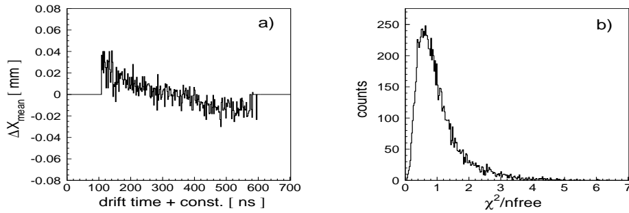
Figure 5.3: (a) Corrections to the time-space relationship. The time-space calibration optimized for one experimental run was used to the data from another run. One observes the change of the drift velocity between these runs. (b) \chi^2 distribution defined in equation 5.1.
