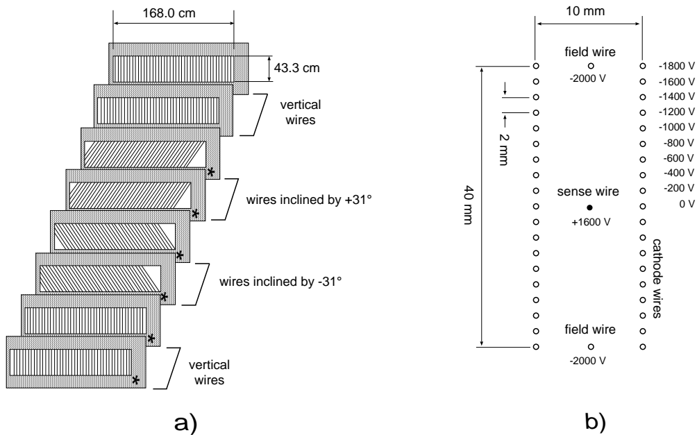
Figure 5.1: (a) Orientation of wires in the drift chamber D2. The smaller drift chamber D1 contains six planes which are indicated by asterisks. (b) Cell structure and voltage distribution. The sense wires are made of 20\mu\text{m} thick gold-plated tungsten, and for the field and cathode wires 50\mu\text{m} Cu-Be was used. Pictures a) and b) are taken from [17].
