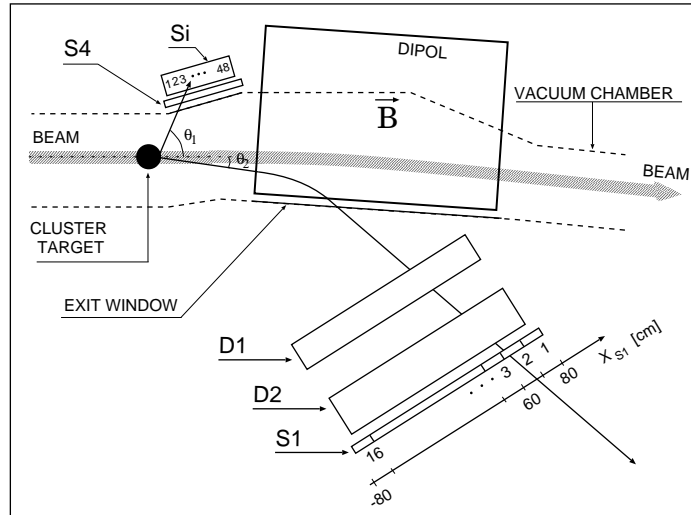
Figure 7.1: Schematic view of the COSY-11 detection setup. Only detectors used for the measurement of the elastically scattered protons are shown. Compare Figure 4.1 on page 24 and also Figure 5.9 on page 36. Numbers, at the silicon detector (Si) and below the S1 counter, indicate the order of pads in the silicon detector (Si) and of segments in the S1 counter, respectively. The X_{S1} axis is defined such that the first segment of the S1 ends at 80 cm and the sixteen segment ends at -80 cm.
