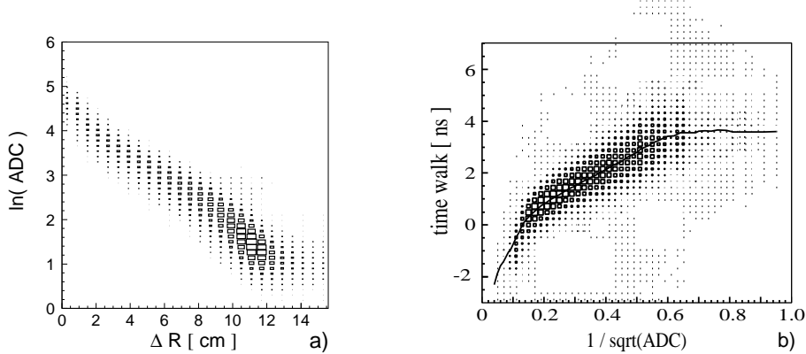
Figure 5.7: (a) A natural logarithm of the ADC value normalized to the path length in the scintillator, in arbitrary units, as a function of a distance between the photomultiplier and the position where particle crossed the scintillation wall. The picture was done for protons with velocities in the range of [0.73 \cdot c : 0.77 \cdot c] . (b) Time walk effect in the S3 detector. Difference between TOF measured between S1 detector and a chosen photomultiplier in the S3 detector and TOF calculated from the reconstructed particle momentum as a function of the inverse of the square root of the signal charge ( \frac{1}{\sqrt{ADC}} ) in the studied photomultiplier. The line shows the mean time walk values calculated for each ADC channel, \frac{1}{\sqrt{ADC}} is given in arbitrary units.
