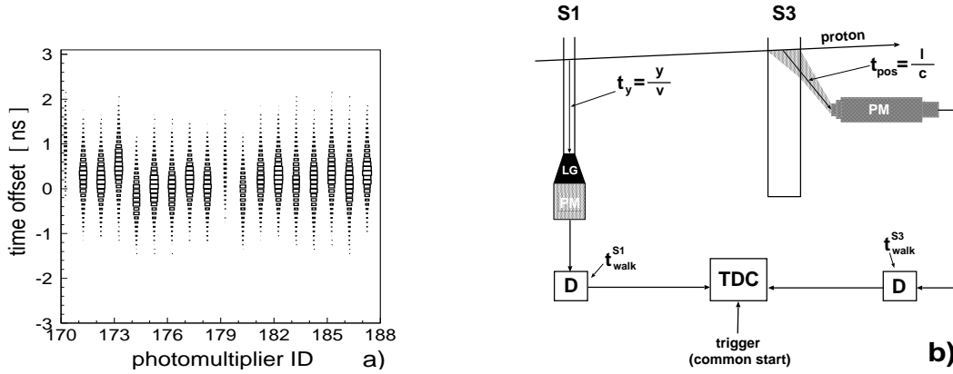
Figure 5.8: (a) The same time difference as in Figure 5.7b, but after the time walk correction, versus a photomultiplier ID of the S3 scintillator. The picture shows offsets only for two columns of photomultipliers. Note that the photomultipliers with numbers 170 and 179 have registered essentially less events than others. This is because they are positioned at the upper and lower scintillator edge (see Figure 5.6). (b) Principle of the time-of-flight measurement between the S1 and S3 scintillation counters. “D” stands for discriminator.
