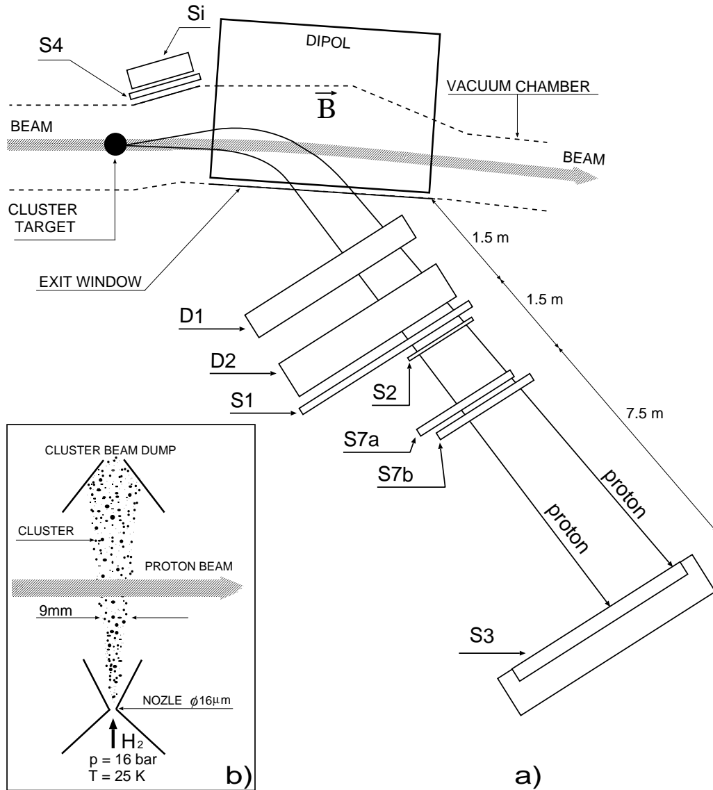
Figure 4.1: a) Schematic view of the COSY-11 detection setup [17]. The cluster target is located in front of the accelerator dipole magnet. Protons from the pp \rightarrow pp\eta' reaction are bent by the magnetic field of the dipole magnet, whereas the beam particles keep circulating in the COSY ring. The decay products of the \eta' meson are not shown, since the analysis is based on the measurement of the four-momenta of the outgoing protons. Shown tracks indicate the space limits expected for the protons ejected after the pp \rightarrow pp\eta' reaction at a beam momentum of 3.222 MeV/c. The produced protons leave the vacuum chamber through the thin exit foil and are detected: i) in two drift chamber stacks D1, D2, ii) in the scintillator hodoscopes S1, S2, S7, iii) and in the scintillator wall S3.
