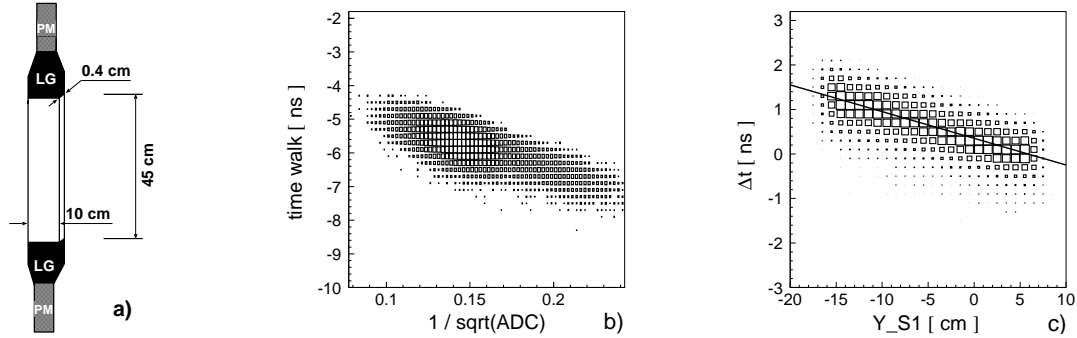
Figure 5.5: (a) Schematic view of a separate scintillation segment of the S1 detector. LG stands for light guide and PM for photomultiplier. (b) An example of the time walk effect for the upper part of one module of the S1 detector. \frac{1}{\sqrt{ADC}} is given in arbitrary units. The time walk values are negative because of the still wrong time offsets at this stage of the analysis (see next section). (c) The velocity of the light signal in the S1 scintillator. The same time difference as in b), but after a time walk correction, versus the vertical position in the S1 detector.
