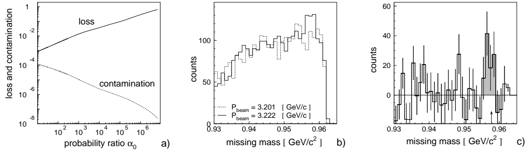
Figure 9.6: (a) Contamination - the probability of accepting the hypothesis that two particles cross the detector when it is false. Loss - probability of rejecting the hypothesis that two particles cross the detector when it is true. Both quantities are shown as a function of the probability ratio \alpha_0 defined in the text. The calculations were performed applying equations 9.6 and 9.7. (b) Missing mass spectrum obtained under the assumption that events with the probability ratio \alpha larger than 10^5 are with two close tracks crossing the detectors. The dashed line corresponds to the measurement below threshold at a beam momentum of P_{beam} = 3201 MeV/c and the solid line indicates the measurement above threshold at P_{beam} = 3222 MeV/c (c) Difference between solid and dashed histogram from b).
