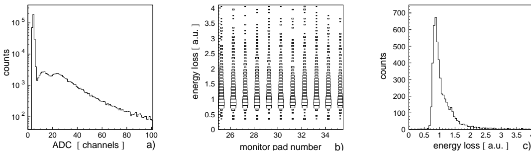
Figure 5.10: (a) Charge (ADC) spectrum from the silicon detector, integrated over all pads. (b) Energy loss measured by means of the silicon pad detector, for the elastically scattered protons, as a function of the pad number. Only ten pads from the middle row of the detector are shown. (c) The normalized energy loss integrated over all pads for the elastically scattered protons. In the analysis it was required that the energy loss must be larger than 0.3 in the units from the picture which corresponds to the ADC value of 7. One observes that this demand has negligible influence on the efficiency.
