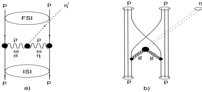
Figure 3.4: Diagrams for the pp \rightarrow pp\eta' reaction near threshold: (a) emission from the virtual particle, (b) production via a fusion of gluons.
