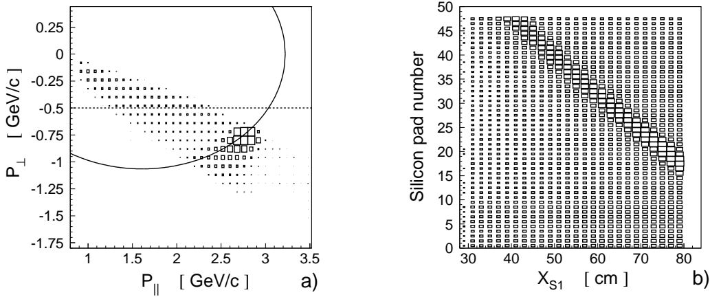
Figure 7.2: (a) Components of the momentum vector of particles registered in both drift chambers and the S1 detector. The momentum component transversal with respect to the beam direction is shown versus the parallel one. The solid line corresponds to the expected dependence between both momentum components for the elastically scattered protons. The dashed line shows the cut performed in the analysis. The shown sample of data was measured at the nominal beam momentum of P_{beam} = 3222 \text{ MeV}/c with the trigger T_{pp} \equiv T_{S1} \wedge T_{S4} . (b) Pad number of the silicon detector versus the position in the S1 detector. Only the data below the dashed line from Figure (a) were taken. Essentially only silicon pads with numbers from 14 to 48 and the S1 segments from 1 to 4 recorded simultaneously elastically scattered protons. Note that the number of entries per bin is given in the logarithmic scale.
