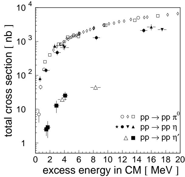
Figure 10.1: Total cross section for the reactions:
