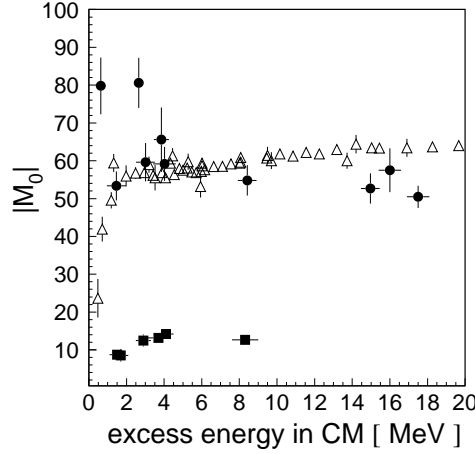
Figure 11.4: Modulus of the dimensionless primary production amplitude M_0 as defined in equation 11.6. The symbols show the results extracted from the experimental data for the reactions pp \rightarrow pp\pi^0 (open triangles) [71, 70, 69], pp \rightarrow pp\eta (filled circles) [78, 20, 138, 79, 139], and pp \rightarrow pp\eta' (filled squares) - data from this work and reference [20].
