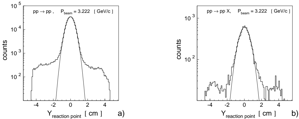
Figure 9.1: The distribution of the vertical component of the reaction point obtained in the experiment for the beam momentum of 3222 \text{ MeV}/c . The solid line shows the fitted Gaussian distribution.
