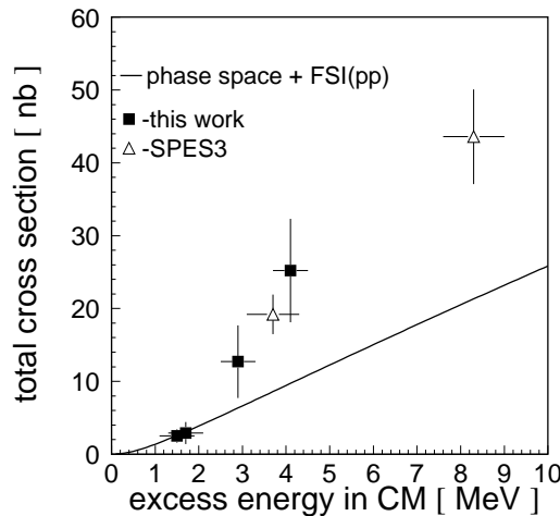
Figure 11.1: Energy dependence of the total cross section as given by the phase space factors and the proton-proton final state interaction (solid line). The experimental values of the total cross section for the pp \rightarrow pp\eta' reaction are indicated by filled squares (this work) and by open triangles (SPES3 [20]). The shown errors take account of both statistical and systematical uncertainties.
