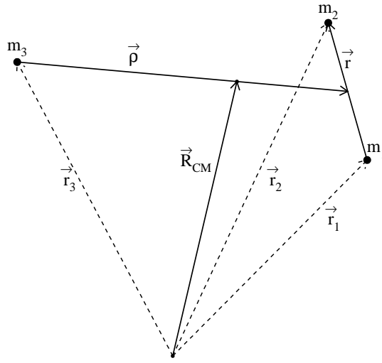
Figure E.1: Definition of the Jacobi coordinates system
