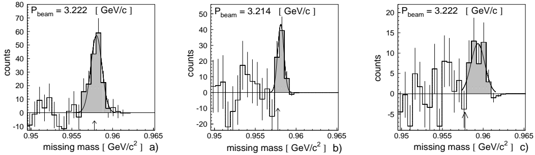
Figure 8.1: (a) Missing mass spectrum measured with the COSY-11 beam optics at a constant nominal beam momentum of 3222 MeV/c . The shaded area corresponds to events assigned to the \eta' meson production. The fit of the Gaussian distribution to the data is shown as the solid line. The arrow indicates the \eta' meson mass.
