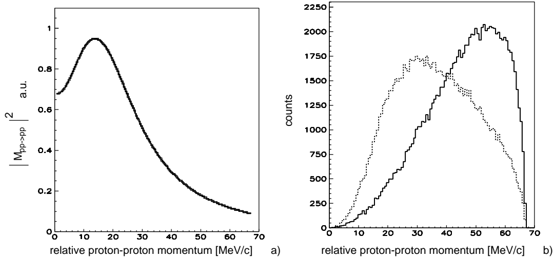
Figure C.1: (a) Square of the proton-proton scattering amplitude as a function of the centre-of-mass momentum. (b) Relative proton-proton momentum distribution for the pp \rightarrow pp\eta' reaction as given by the phase-space without proton-proton FSI - solid line, and with proton-proton FSI - dotted line.
