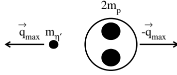
Figure F.1: The produced meson has a maximum momentum if both protons are emitted with the same momentum vector.
