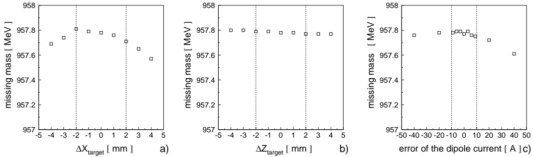
Figure 8.3: (a) The reconstructed missing mass versus the deviation of the target position in the horizontal direction perpendicular to the beam axis. The position of the target is known with an accuracy better than \pm 2\text{ mm} which corresponds to the missing mass variation smaller than \sim 0.1\text{ MeV} . (b) Missing mass versus the deviation of the target position along the beam direction. Since the position of the target is known to be better than \pm 2\text{ mm} the missing mass variation caused by this parameter is less than \sim 0.04\text{ MeV} . (c) Missing mass versus changes of the dipole current. The absolute current value used in the measurement of the pp \rightarrow pp\eta' reaction was \sim 3700\text{ A} which corresponds to the vertical magnetic field component of \sim 1.53\text{ T} . The magnetic field is known with the accuracy better than 0.25\% which is equivalent to a missing mass variation of less than \sim 0.06\text{ MeV} .
