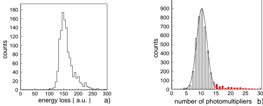
Figure 6.3: (a) Energy loss distribution measured in a segment of the S1 detector obtained for events with two protons having velocities in the range between 0.7 c and 0.8 c , both crossing through the same segment. Units on the horizontal-axis are the same as in Figures 6.2a and 6.2b. (b) Number of photomultipliers (multiplicity) giving signals in the S3 detector, for two protons with velocities in the range between 0.7 c and 0.8 c crossing the scintillation wall. The line shows the Gaussian distribution fitted to the data. The shaded tail corresponds to events when at least one proton made a nuclear reaction in the scintillator.
