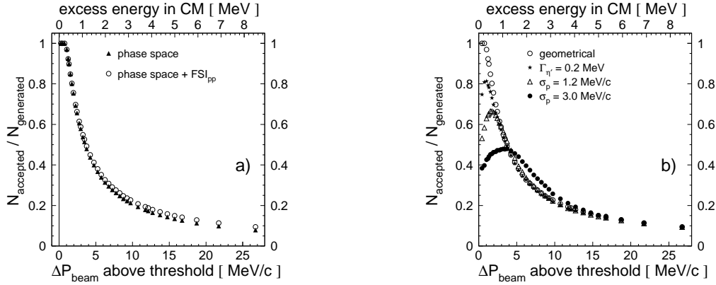
Figure 9.3: Efficiency of the detection system for the pp \rightarrow pp\eta' reaction as a function of the beam momentum above threshold (lower axis), or as a function of the excess energy (upper axis)
