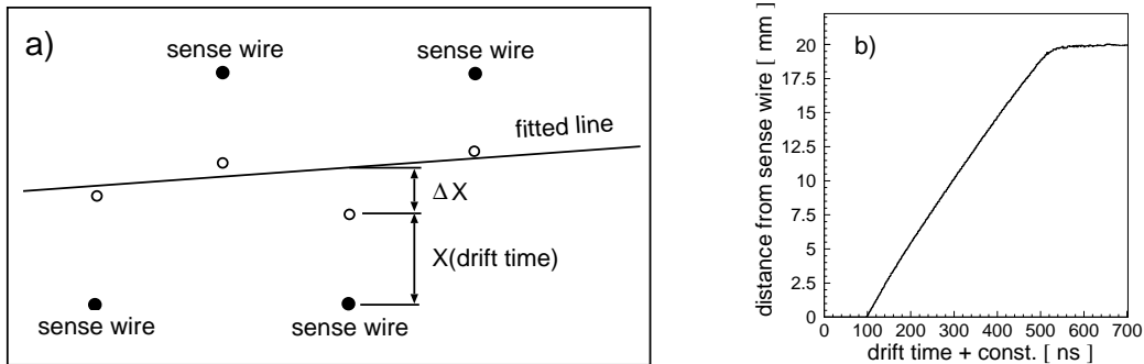
Figure 5.2: (a) Principle of the correction of the time-space calibration. X denotes the distance from the sense wire obtained from the measured drift time applying the time-space calibration. (b) Time-space calibration i.e. relationship between the distance from the sense wire and the drift time.
