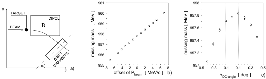
Figure 8.2: (a) Schematic view of the relative settings for the target, the dipole magnet and the drift chamber stack at the COSY - 11 detection system. (b) Offset of the absolute beam momentum transfers linearly to the the missing mass, namely as: 3 \cdot \Delta P [\text{MeV}/c] \simeq \Delta mm [\text{MeV}] . (c) Missing mass of the \eta' meson as a function of the error of establishing the drift chamber angle. This angle is known with an accuracy better than \pm 0.1^\circ where the missing mass changes by less than \sim 0.15 \text{ MeV} . The results of b) and c) were obtained by means of the Monte Carlo method.
