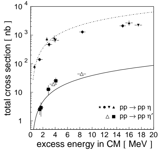
Figure 11.2: Total cross section for the pp \rightarrow pp\eta and pp \rightarrow pp\eta' reactions as a function of the excess energy Q .
