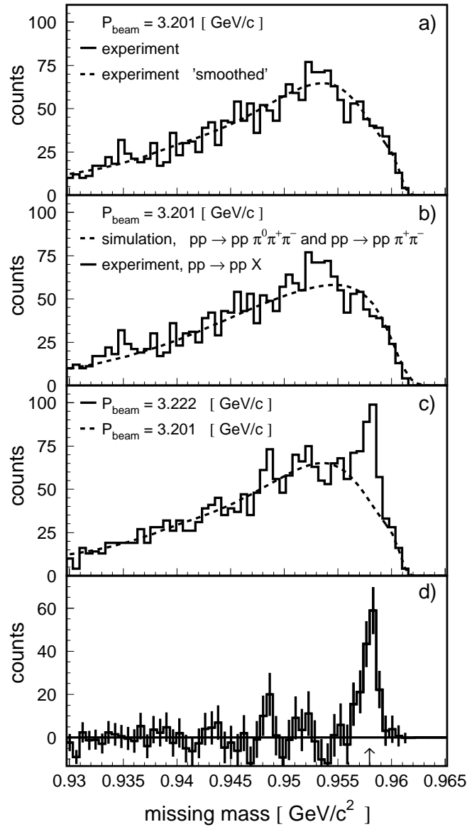
Figure 6.5: Missing mass of the unobserved particle or system of particles in the pp \rightarrow ppX reaction.
