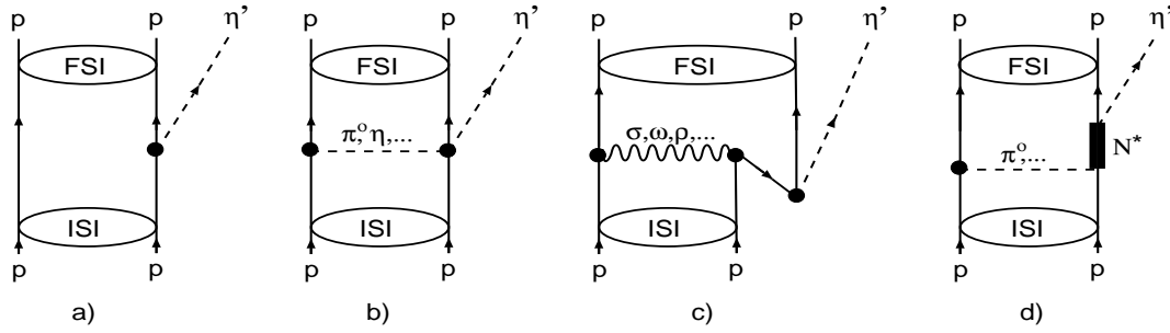
Figure 3.3: Feynman diagrams for the pp \rightarrow pp\eta' reaction near threshold: (a) direct term, (b) “rescattering” term, (c) production through the heavy-meson exchange, (d) excitation of an intermediate resonance.
