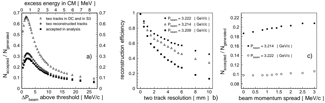
Figure 9.4: (a) Simulated efficiency of the detection system as a function of the beam momentum above threshold (lower axis), or as a function of the excess energy (upper axis). The triangles are the same as in figure 9.3b. Stars indicate the ratio of the number of events for which both proton trajectories were reconstructed to the number of all generated events. The solid squares indicates the ratio of the number of events which fulfilled all requirements demanded in the analysis to the number of all generated events. (b) Efficiency of the two track reconstruction as a function of the two-track-resolution of the drift chambers. The two-track-resolution was estimated to be 3.0 \text{ mm} \pm 1.0 \text{ mm} , where the error of \pm 1.0 \text{ mm} causes the inaccuracy of the reconstruction efficiency of about \pm 8\% . (c) The overall detection efficiency as a function of the beam momentum spread for the nominal beam momentum of P_{\text{beam}} = 3222 \text{ MeV}/c and P_{\text{beam}} = 3214 \text{ MeV}/c . Taking the beam momentum spread of 1.2 \text{ MeV}/c with the accuracy of \pm 0.1 \text{ MeV}/c one obtains the changes of the detection efficiency of \pm 0.5\% .
