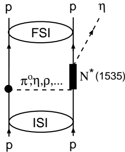
Figure 3.2: Dominant term for the pp \rightarrow pp\eta production amplitude.
