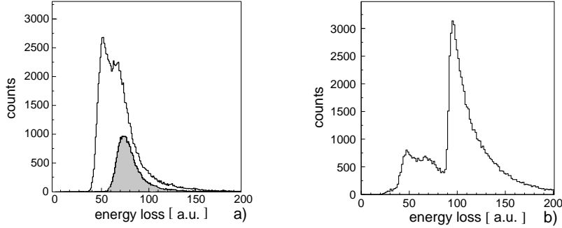
Figure 6.2: (a) Energy loss distribution in a segment of the S1 detector measured with a test trigger ( T_{s1,\mu=1} \wedge T_{s3,\mu>2} ). Values on the horizontal-axis correspond to the sum of the ADC values from upper and lower photomultiplier. Two peaks originate from pions and protons. The shaded histogram corresponds to protons with the velocity in the range between 0.7c and 0.8c . Producing this spectrum exactly one track in the drift chambers was required. (b) Energy loss distribution in a segment of the S1 detector obtained with the T_{\eta'} trigger. If the trigger is released by the S2 detector or two particles cross separate segments in the S1 then, in each segment separately, the same structure as in a) is observed. However, if only one segment has a signal, then it is required (by the electronics - compare Figure 6.1) that the sum of the pulse charges from the upper and the lower readout must be larger than the threshold value, which is in this case equal to ninety.
