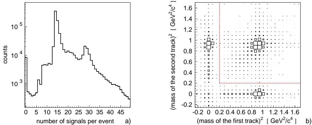
Figure 6.4: (a) Number of signals from drift chambers per event. A sample of data from a six hours measurement is shown. The D1 and D2 drift chambers have together fourteen planes. Thus, peaks with maxima at 14 and 28 number of signals per event correspond to one and two particles crossing the chambers, respectively. The enhancement at 42 corresponds to three particles. A small peak at 6 originates from one particle which passed through the insensitive area in the planes with inclined wires (compare Figure 5.1). Similarly, an enhancement at 20 corresponds to two particles from which one passed through this area. The peak in zero appears because the trigger detector S1 is larger than the drift chamber active area. (b) Squared masses of two particles measured in coincidence. The pronounced peak close to the centre of the figure corresponds to two registered protons. Peaks are recognized also when proton and pion or two pions were detected.
