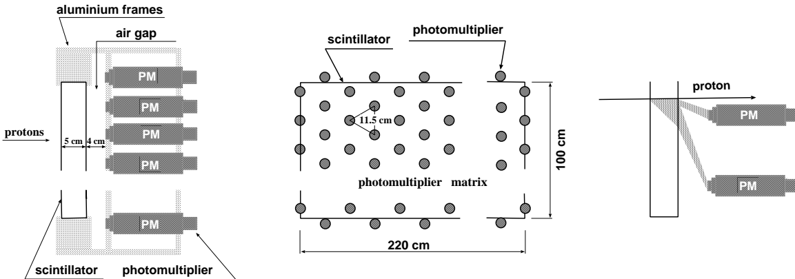
Figure 5.6: Schematic view of the S3 scintillation detector. A side view (left part). The photomultiplier matrix together with the dimensions of the scintillation wall (middle part). Principle of the light collection (right part).
