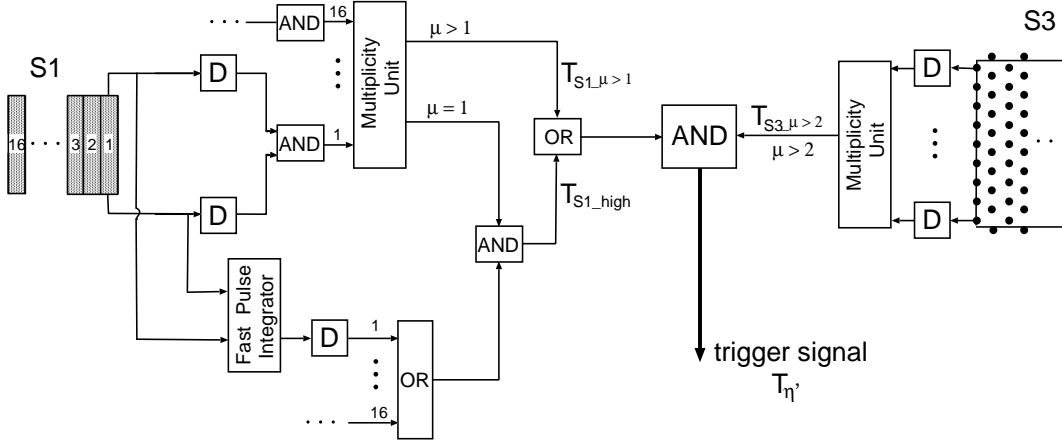
Figure 6.1: Simplified scheme of the trigger electronics for the detection of two outgoing charge particles. The S2 detector, not shown here, is connected identically as the S1 counter. In the case of the S1 detector the multiplicity unit defines the number of segments which have a signal, and in the case of the S3 detector the number of active photomultipliers is determined. For more details of the trigger electronics see [114, 117].
