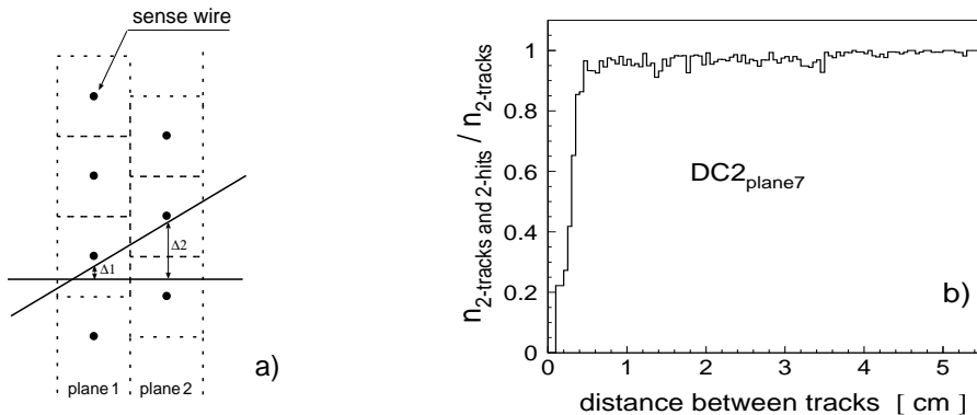
Figure 5.4: (a) A schematic view of two subsequent planes of the drift chamber. If the distance between two tracks in a given plane is smaller than some minimum value, then only one signal will be detected on the sense wire in this plane. (b) The number of events with two tracks and two hits divided by the number of events with two tracks as a function of distance between tracks in the seventh plane of the drift chamber D2.
