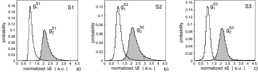
Figure 9.5: Energy loss spectra for one and two particles crossing the scintillation detectors. The energy loss is normalized to the expected energy loss for one particle obtained from the known stopping power and the path length in the scintillator. The shaded histogram corresponds to two particles crossing the detector. The number of entries per energy bin was normalized so that the sum over all bins is equal to 1.
