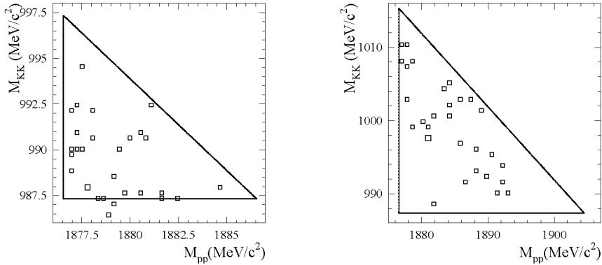
FIGURE 4. Goldhaber Plots obtained from measurements [8] at Q = 10 MeV (left) and Q = 28 MeV (right). Solid lines show boundaries of the physically allowed region at appropriate excess energies.
