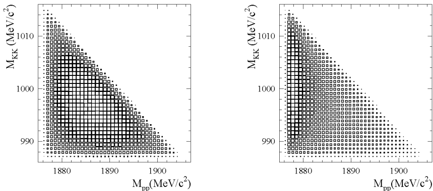
FIGURE 3. Monte Carlo simulations of the pp \rightarrow ppK^+K^- reaction at Q = 28 MeV: (left) Goldhaber plot for a homogeneously populated phase space; (right) Phase space density distribution modified by proton-proton final state interaction.
