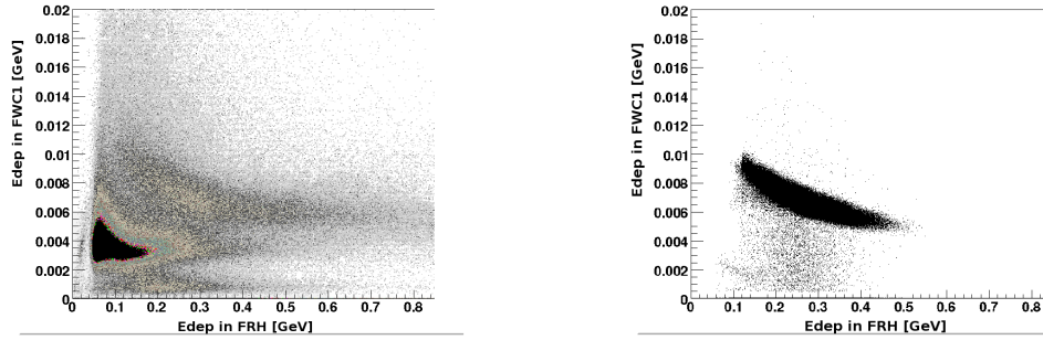
Fig. 3. Energy loss in the Window Counter as a function of the energy loss in the Forward Range Hodoscope as obtained in the experiment (left), and as simulated for the {}^3\text{He} ions outgoing from the dd \rightarrow ({}^4\text{He}\eta)_{\text{bound}} \rightarrow {}^3\text{He}p\pi^- reaction (right).
