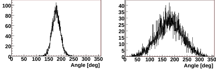
Fig. 1. Distribution of the relative p - \pi angle seen in the reaction center-of-mass system as simulated for the processes leading to the creation of \eta -helium bound state: dd \rightarrow (^4\text{He}\eta)_{\text{bound}} \rightarrow {}^3\text{He}p\pi (left), and for the prompt production of the {}^3\text{He}p\pi system assuming a homogeneous population of the phase space for the dd \rightarrow {}^3\text{He}p\pi reaction (right).
