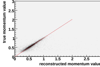
Fig. 4. Monte Carlo: Reconstructed momentum versus true momentum for two charged particles registered in the Central Detector under the condition that a {}^3\text{He} nucleus was detected in the Forward Detector
