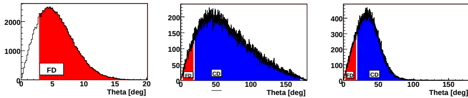
Fig. 2. Angular distributions of {}^3\text{He} (left), pions (middle) and protons (right) outgoing from the dd \rightarrow (^4\text{He}\eta)_{\text{bound}} \rightarrow {}^3\text{He}p\pi reaction. Labels "FD" and "CD" indicate angular ranges covered by the Forward Detector and Central Detector, respectively. Please note that the presented range for {}^3\text{He} ions is smaller than those for protons and pions.
