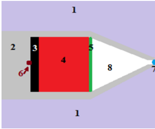
Figure 50. Scheme of one of the simulated Beam Shaping Assemblies (BSA #14): Concrete shielding (purple)(1), 20 cm thick back and 10 cm thick side Pb reflectors (gray) (2), 8cm thick ^{186}\text{W} (black) (3), 45 cm thick mixture of Fe(5%) \text{AlF}_3 (95%) (red) (4), 1.25 cm thick Cd (green) (5), neutron source hollow (dark red) (6), R = 2.5 cm virtual sensitive detector (blue) (7) and vacuum (8) is inside the lead collimator (white).
