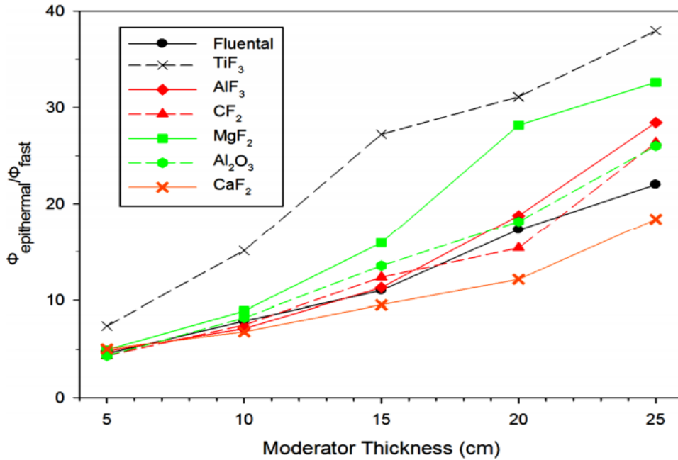
Figure 32. Epithermal over fast neutron flux ratio dependence for various materials and thicknesses installed next to {}^7\text{LiF} as second part of moderator (for the BSA in the Figure 34) (Figure adopted from J. Fantidis and A. Antoniadis 2015)
