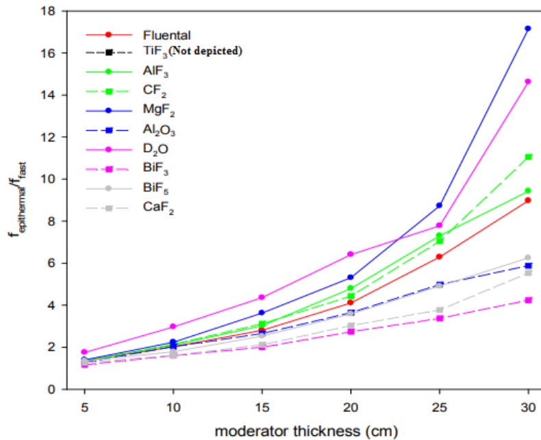
Figure 21. Epithermal over fast neutron flux ratio as a function of thickness of various materials installed next to TiF_3 as second part of moderator (Figure adopted from J. Fantidis et al 2013).
