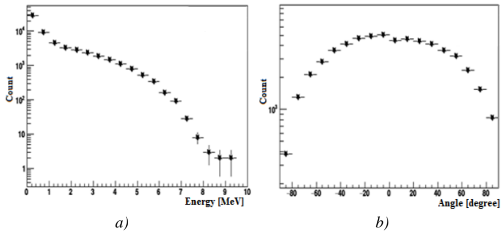
Figure 48. Energy (a) and angular (b) distribution of gamma rays after the BSA shown in Figure 45. The spectra were obtained based on 10^8 simulated events.
