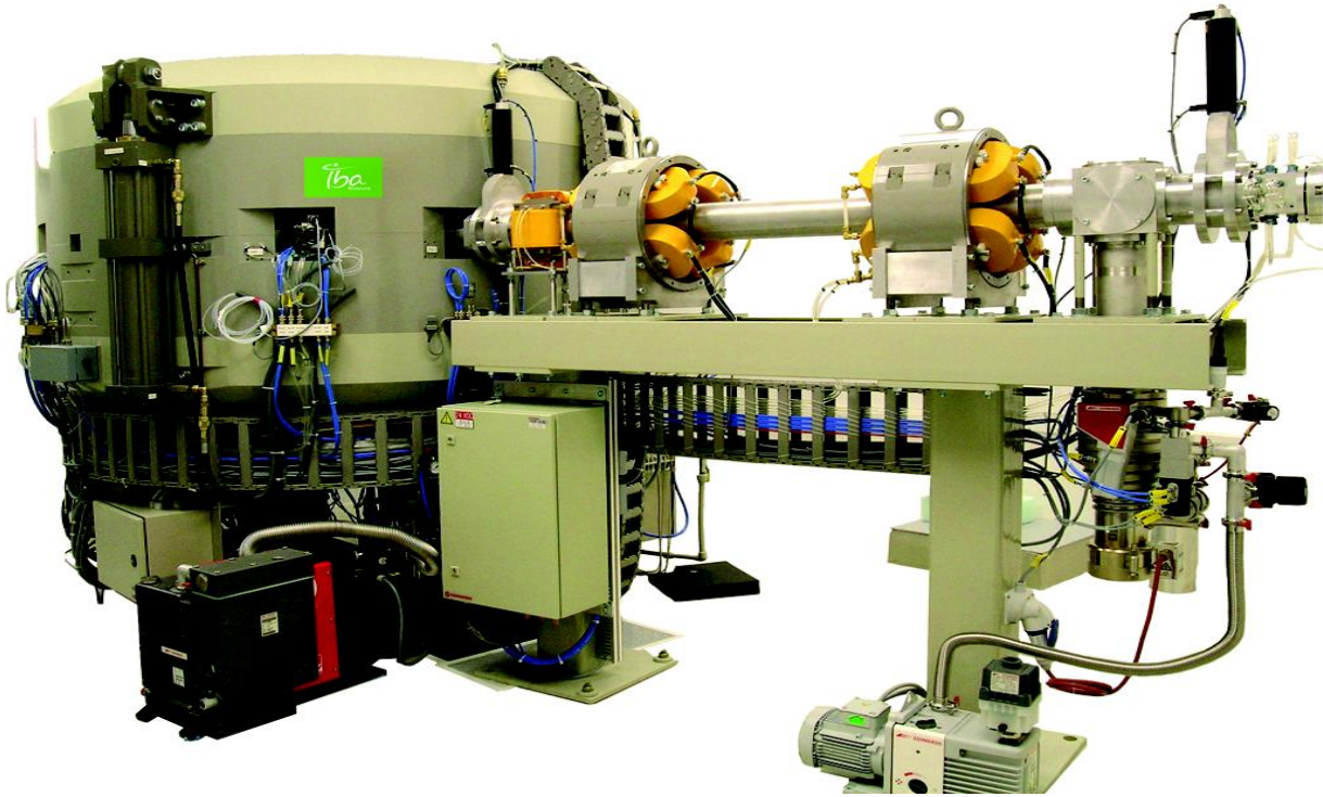
Figure 41. A photo of the C18/18 cyclotron of IBA with proton beam transport line (Adopted from IBA brochures, see the link in the references).
