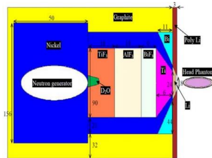
Figure 24. Geometric configuration of the BNCT system not in scale (dimensions are given in cm) (Figure adopted from Fantidis et al. 2013).
