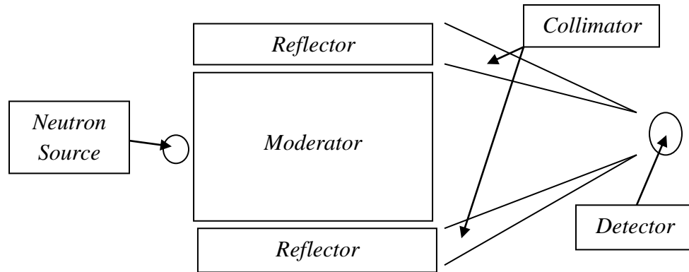
Figure 11. Main parts of the BSA with additional components needed for the experimental setup.
