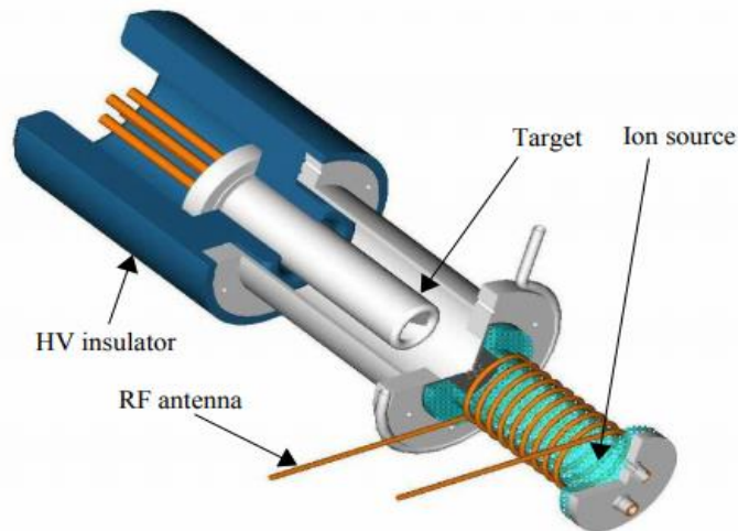
Figure 7. The axial extraction neutron generator (Figure adopted from T. Pui Lou 2003).
