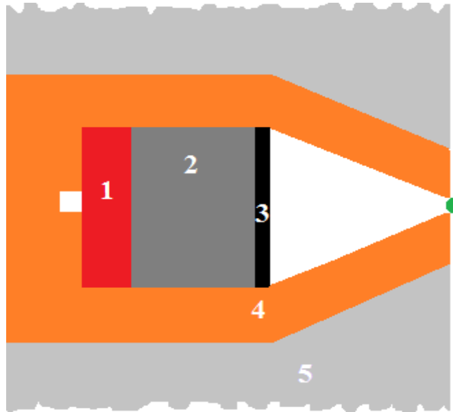
Figure 56. Scheme of the BSA based on DT neutron generator. As listed in Table 7 moderator parts are numbered (1), (2) and Filter (3), while in Table 8 with same scheme of the BSA Multiplier (1), Moderator (2) and Filter (3) are listed. In both cases 20 cm thick lead side and back reflectors as well as collimator with same material and thickness (4) were simulated. For shielding purposes the BSA is placed in a concrete wall (5).
