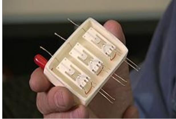
Figure 8. World’s smallest CNGs (neutrusters) of Sandia National Laboratories mounted in a test box under vacuum (max yield is ~200 n/s per neutruster, Figure adopted from Sandia National Laboratory (see the link at references)).
