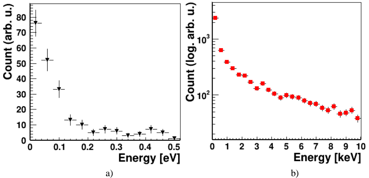
Figure 53. Energy distributions of (a) thermal and (b) epithermal neutrons obtained in the case of BSA #20.
