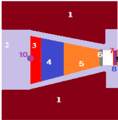
Figure 52. Scheme of the purely conical BSA #20 inside of the concrete wall (1) with back and side lead reflectors and in air lead collimator (filters placed inside of the tube-collimator) (2), 10 cm thick W (3), 15 cm \text{Fe}_2\text{O}_3 (4), 35 cm Al (5), 1.25 cm thick LiF (6), 1 mm thick Bi (7), 1 mm thick Pb outlet window (8), virtual sensitive detector ( D = 12 cm) (9) and neutron source hollow (10) with 1 \text{ cm}^3 volume.
