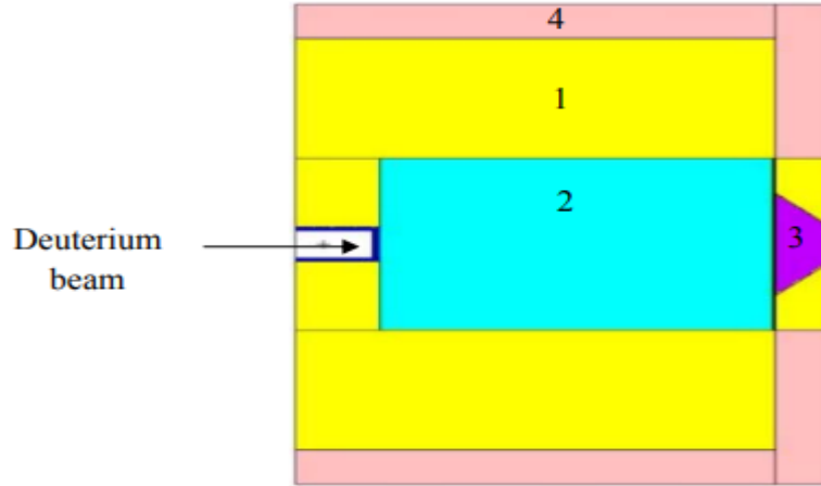
Figure 27. DD based BSA configuration with (1) reflector, (2) moderator, (3) collimator and (4) gamma shield (Figure adopted from Y. Kasesaz et al. 2013).
