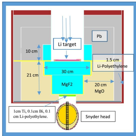
Figure 15. Final design of the BSA used at the Russian BNCT laboratory in Novosibirsk (Figure adopted from (L. Zaidi et al. 2018)).
