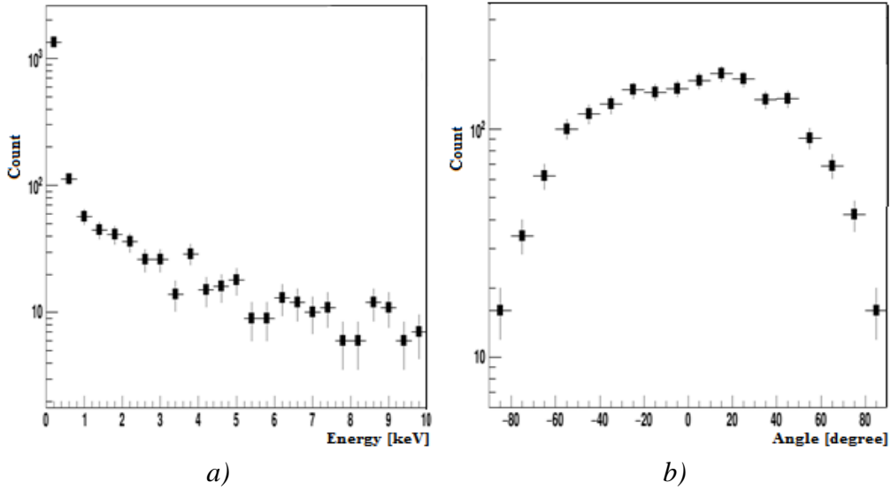
Figure 47. Energy (a) and angular (b) distribution of epithermal neutrons after the BSA shown in Figure. 46. The spectra were obtained based on 10^8 simulated events
