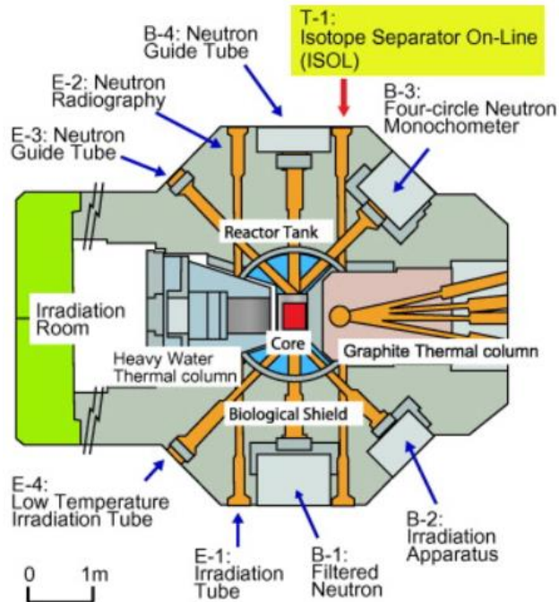
Figure 13. Schematic view of the KUR reactor (Figure adopted from A. Taniguchi et al. 2013).
