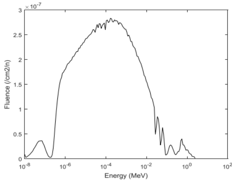
Figure 26. Energy distribution of neutrons registered at the beam aperture (For the BSA presented in Figure 25) (Figure adopted from M. Hsieh et al. 2017).
