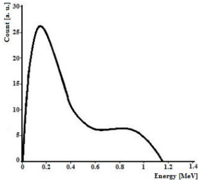
Figure 44. Simulated neutron spectrum detected by 10 cm diameter virtual sensitive detector placed on the exit of the BSA. As presented in Figure 43 it is modeled from 5 cm Bi, 55 cm Fe, 10 cm Al, 5 cm graphite and 10 cm Li 7 F with Pb reflector. (Figure adopted from R. Avagyan, V. Ivanyan et al. 2017).
