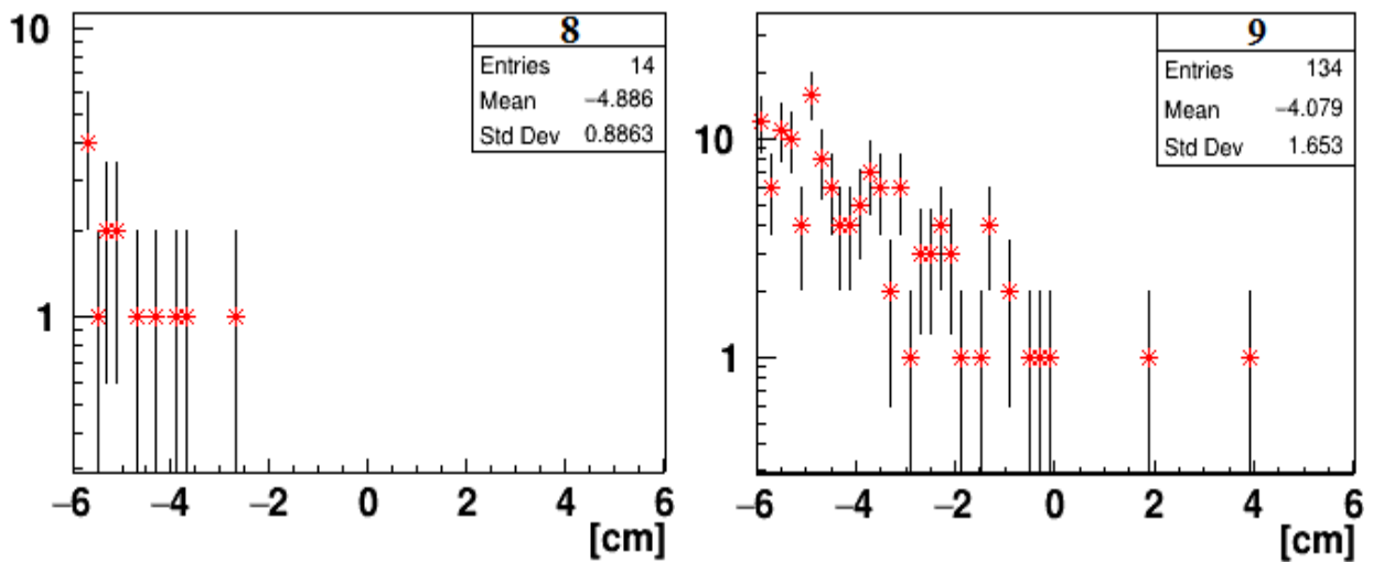
Figure 62. Neutron induced reactions occurred at different depths in the soft tissue with number of neutron reactions (each represents also one neutron participating in the reaction) as function of the penetration depth. Initial energies for separately simulated neutrons in the energy range from 100 keV (label 8) to 1 MeV (label 9) .
