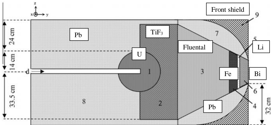
Figure 35. The Scheme of the Optimized BSA based on DT neutron generator, with 14 cm radius of Uranium multiplier (1), 23 cm thick TiF_3 (2), 36 cm thick Fluental (3), 4 cm thick Fe (4), 1 mm thick Li (5), 2.6 cm thick Bi (6), Pb as collimator (7) and reflector (8), with front shield (9) (Figure adapted from F. S. Rasouli 2012).
