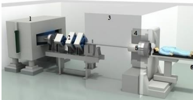
Figure 6. World's first accelerator based BNCT equipment with accelerator (1) beam transport line (2) a concrete wall (3) (separating the patient room (6)) with placed in beam shaping assembly (4) and an appropriate target (5) (Figure adapted from T. Mitsumoto et al. 2010)
