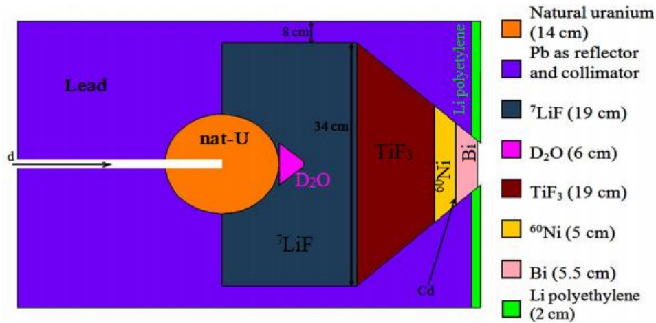
Figure 34. Optimized version of the BSA based on DT neutron generator (Figure adopted from J. Fantidis and A. Antoniadis 2015)
