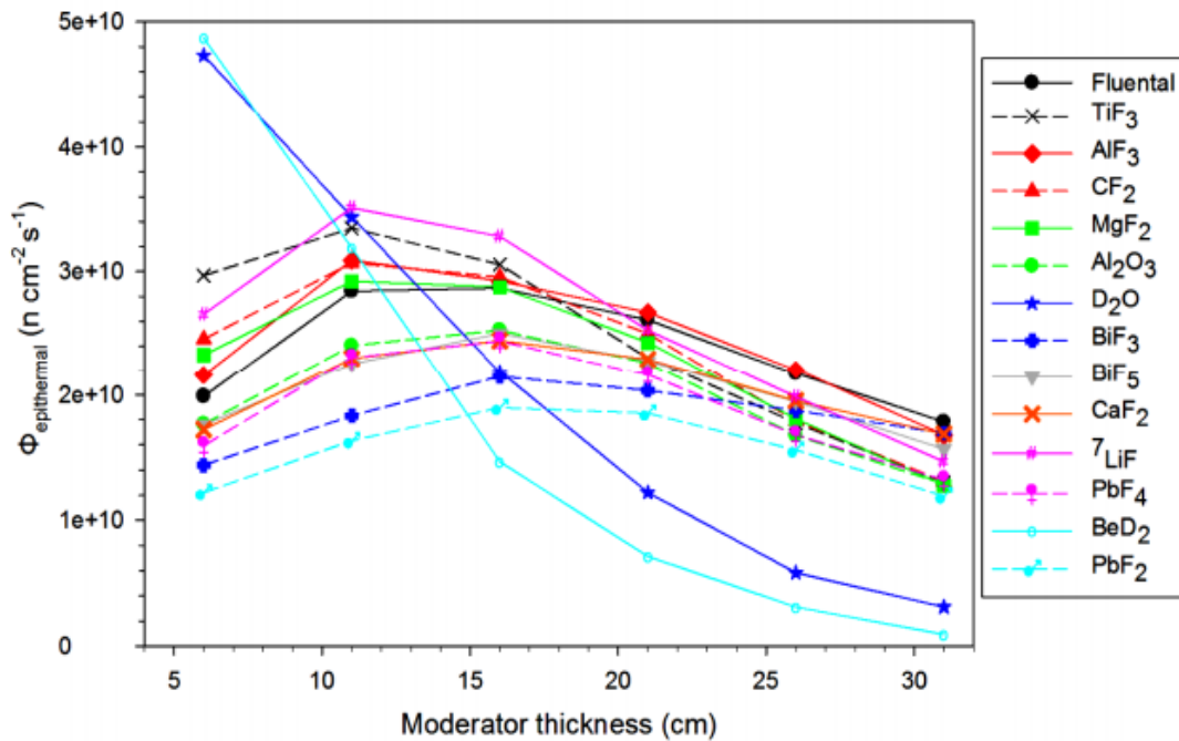
Figure 29. Epithermal neutron flux after first part of moderator (for the BSA in Figure 34) (Figure adopted from J. Fantidis and A. Antoniadis 2015).
