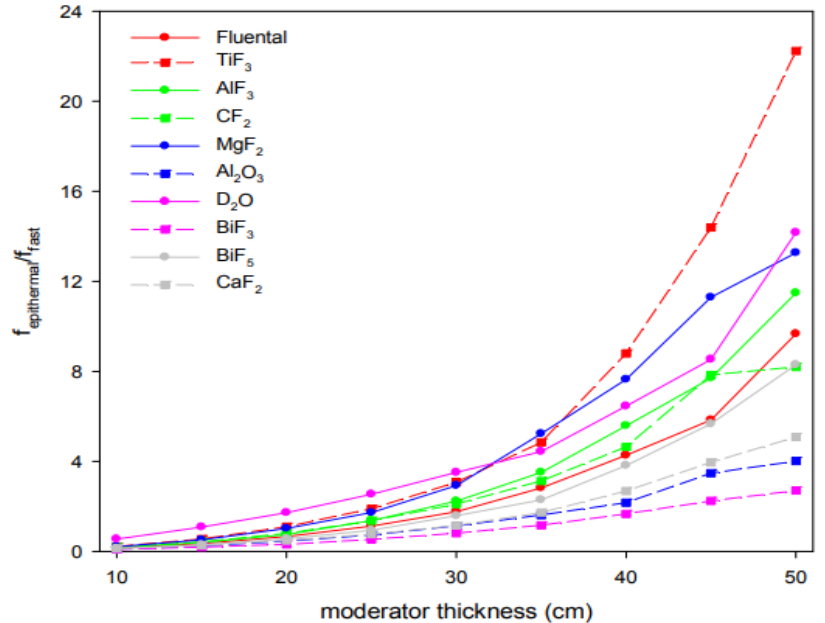
Figure 18. Epithermal over fast neutron flux ratio as a function of thickness of various materials (Figure adopted from J. Fantidis et al 2013).
