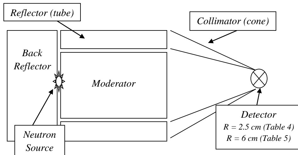
Figure 49. General scheme of a DD CNG based BSA with its main components where the hollow for the point source is 1 \text{ cm}^3 tube. Thicknesses and materials of the BSA designing components were varied to obtain the optimal neutron flux characteristics.
