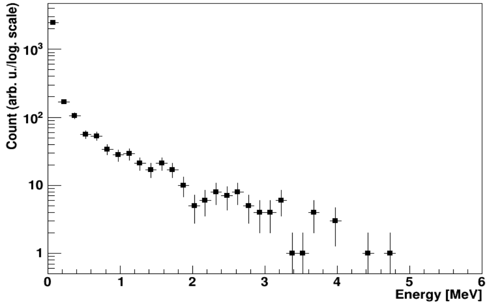
Figure 46. Energy distribution of neutrons after the BSA of 20 cm thick nat-Mo, 45 cm thick nat-Fe and 45 cm thick paraffin boric acid moderator as shown in Figure 20, simulated after the bombardment of 2.5 mm ^9\text{Be} by protons. (Figure adopted from (V. Ivanyan 2020)).
