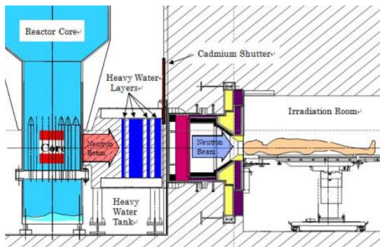
Figure 10. Reactor based BNCT with a BSA made from heavy water layers of neutron moderator in JRR-4 (Figure adopted from (E. Bavarnegin et al. 2017)).
