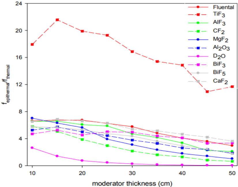
Figure 17. Epithermal over thermal neutron flux ratio as a function of thickness of various materials (Figure adopted from J. Fantidis et al 2013).
