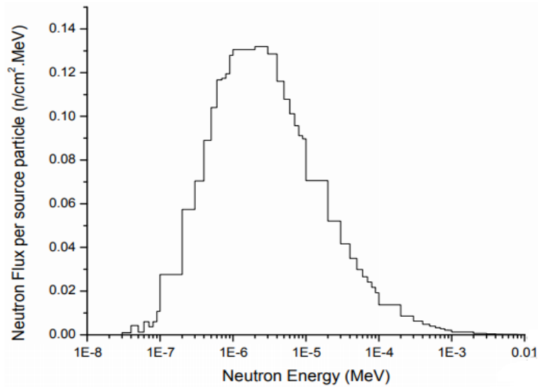
Figure 28. Neutron energy distribution in case of the optimized BSA (Figure 27) (Figure adopted from Y. Kasesaz et al 2013)
