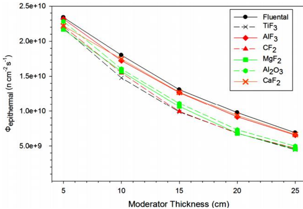
Figure 31. Epithermal neutron flux dependence on various materials and thicknesses as second part of moderator installed next to 7 LiF with conical volume of D 2 O (for the BSA in Figure 34) (Figure adopted from J. Fantidis and A. Antoniadis 2015).
