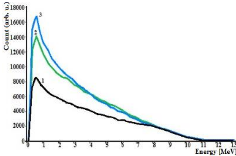
Figure 42. Energy Spectra of neutrons obtained using 0.5 mm (1), 1 mm (2) and 2.5 mm (3) thick ^9\text{Be} (Figure adopted from R. Avagyan, V. Ivanyan et al. 2016).
