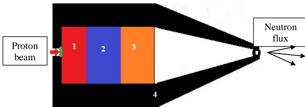
Figure 45. Proton beam (red arrow) bombarding a 2.5 mm thick 9 Be (green) target followed by the BSA consisting of 20 cm thick Mo (1. red), 45 cm Fe (2. blue) and 45 cm paraffin boric acid (3. orange) as moderators, and 20 cm thick Pb (4. black) as reflector ( V. Ivanyan 2020).
