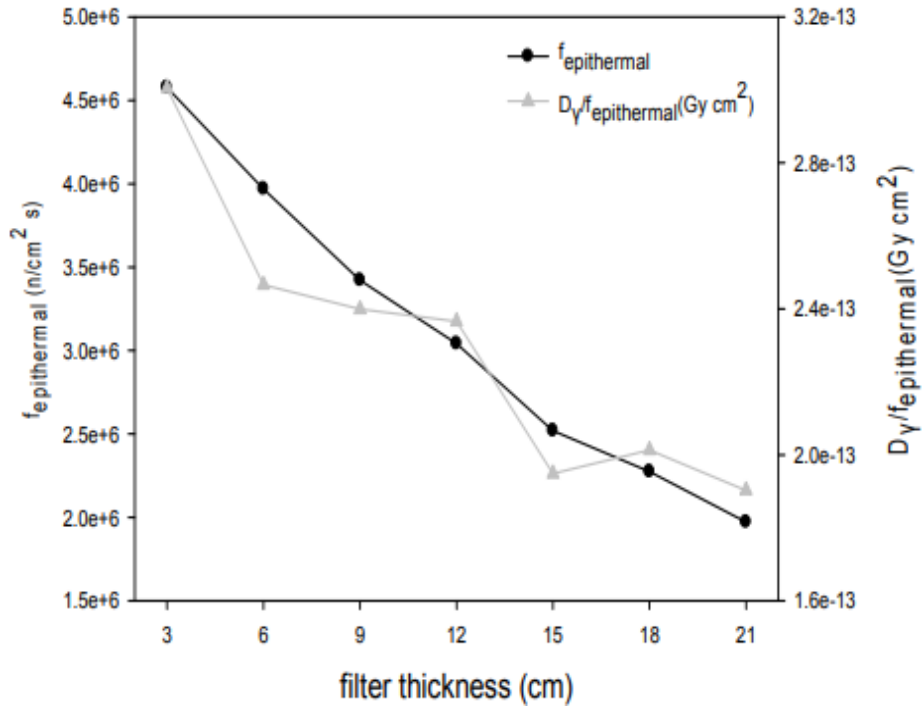
Figure 22. Epithermal neutron flux and D_{\gamma}/f_{\text{epithermal}} (same as D_{\gamma}/\phi_{\text{epi}} ) ratios in case of different thicknesses of Ti filter for the optimized BSA (Figure adopted from J. Fantidis et al 2013).
