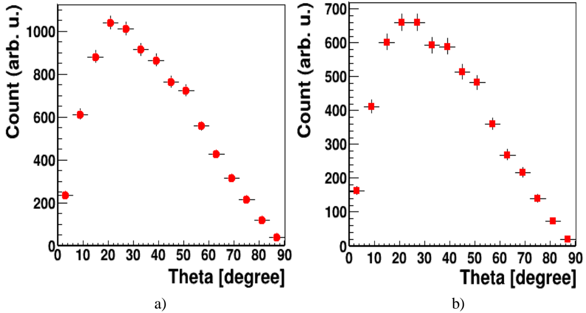
Figure 54. Angular distributions of neutrons in case of the BSA #20. (a) For neutrons with energies up to 2.5 MeV and (b) for neutrons in the energy range from 0.5 eV to 10 keV. The angle is defined with respect to the main axis of the BSA.
