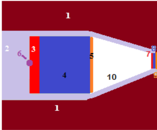
Figure 51. Scheme of the BSA # 15 placed in concrete wall (1) with 20 cm thick back and 10 cm thick side Pb reflectors (2), 8cm thick ^{186}\text{W} (3), 45 cm thick mixture of Fe (5%) and \text{AlF}_3 (95%) (4), 1.25 cm thick LiF (5), 1 cm 3 neutron source hollow (6), 0.5 mm Bi (7), 1 mm Pb outlet window (8), virtual sensitive detector ( D = 12 \text{ cm} ) (9) and vacuum inside of (10) the collimator with same natural Pb material as all of the reflectors .
