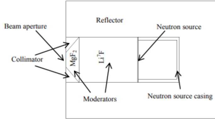
Figure 25. Scheme of the optimized BSA configuration by M. Hsieh et al. (Figure adopted from M. Hsieh et al. 2017).
