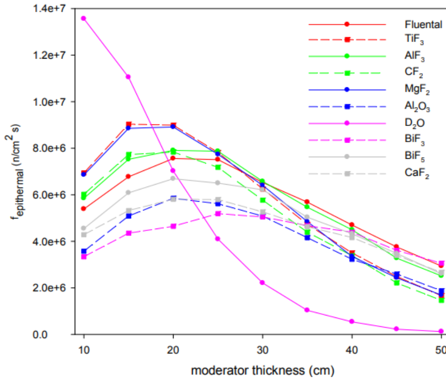
Figure 16. Epithermal neutron flux dependence on various materials and thicknesses (Figure adopted from (J. Fantidis et al 2013) ).
