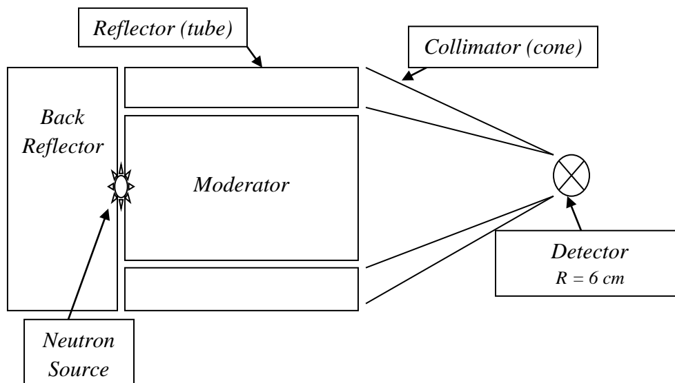
Figure 55. General scheme of a DT CNG based BSA with its main components, where the hollow for the point source is 1 \text{ cm}^3 tube. Thicknesses and materials of the BSA designing components were varied to obtain the optimal neutron flux characteristics.
