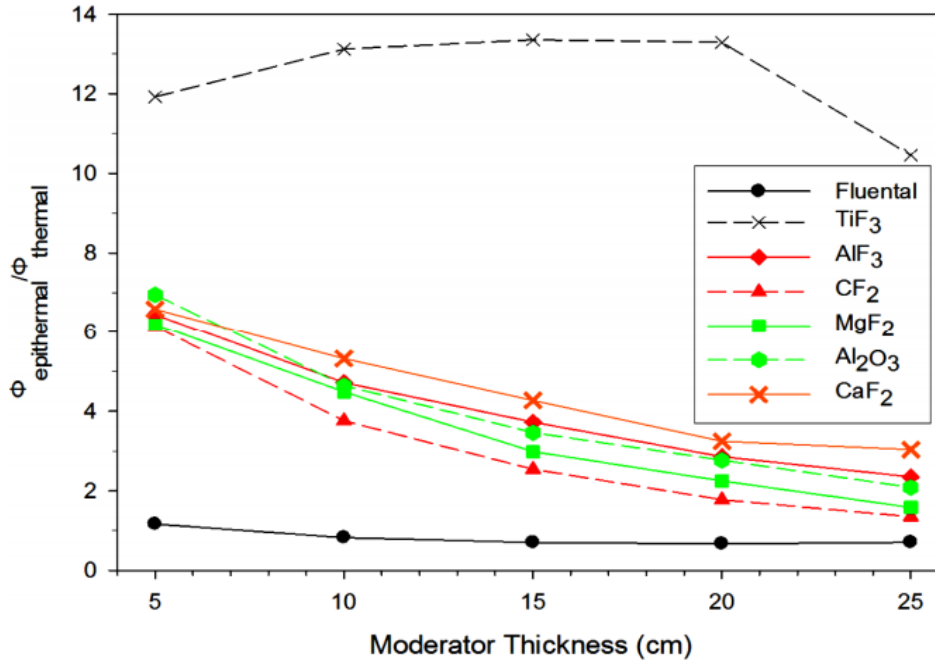
Figure 33. Epithermal over thermal neutron flux ratio dependence for various materials and thicknesses as second part of moderator installed next to {}^7\text{LiF} with conical volume of \text{D}_2\text{O} (for the BSA in Figure 34) (Figure adopted from J. Fantidis and A. Antoniadis 2015)
