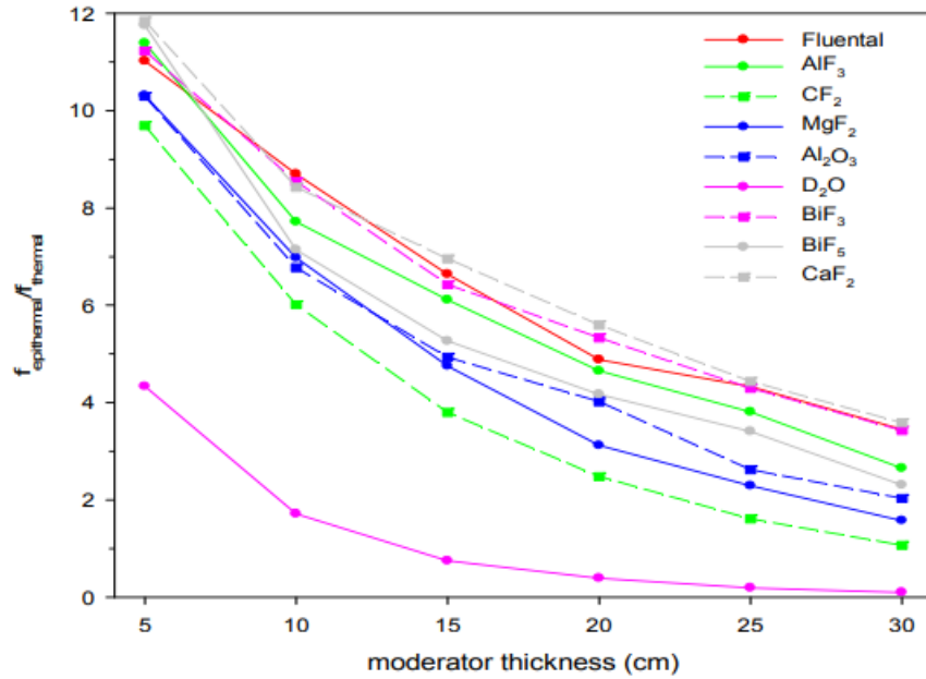
Figure 20. Epithermal over thermal neutron flux ratio as a function of thickness of various materials installed next to TiF_3 as second part of moderator (Figure adopted from J. Fantidis et al 2013).
