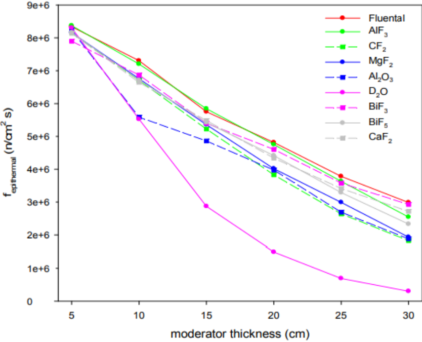
Figure 19. Epithermal neutron flux as a function of thickness of various materials installed next to \text{TiF}_3 as second part of moderator (Figure adopted from J. Fantidis et al 2013).
