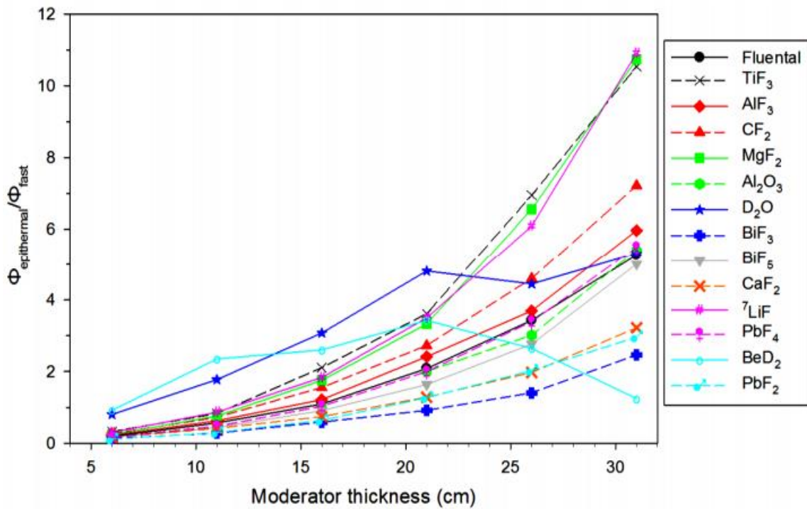
Figure 30. Ratio of epithermal over fast neutron fluxes simulated for different thicknesses and materials for the DT neutron generator used as a source for BNCT (Figure adopted from Fantidis & Antoniadis 2015).
