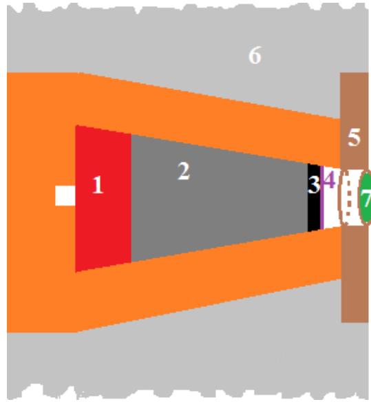
Figure 57. Scheme of the BSA based on DT neutron generator. As listed in Table 9 and 10 with multiplier or first part of the moderator (1), second part of the moderator (2) with last part of the moderator (3) with filters (4). Collimator is Lead or LiF (Table 9) (5) with virtual sensitive detector (7) at the exit window. The system is placed in a concrete wall (6).
