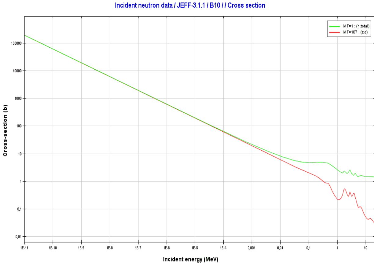
Figure 1. Comparison of the total cross-section (green curve) and cross-section for neutron capture reactions (n, alpha) (red curve) on ^{10}\text{B} (calculated by JANIS code).
