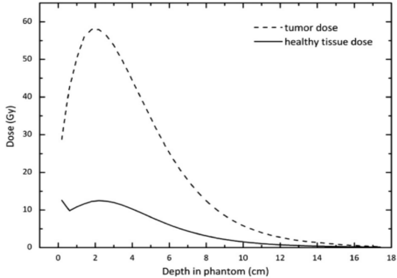
Figure 39. Dose delivery dependence on the depth in tumor and in healthy tissue (Figure adopted from Rasouli et al 2012)
