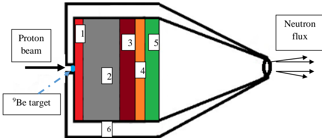
Figure 43. BSA with 2.5 mm 9 Be target, 5 cm Bi (1), 55 cm Fe (2), 10 cm Al (3), 5 cm graphite (4), 10 cm 7 LiF (5), Pb reflector (6).
